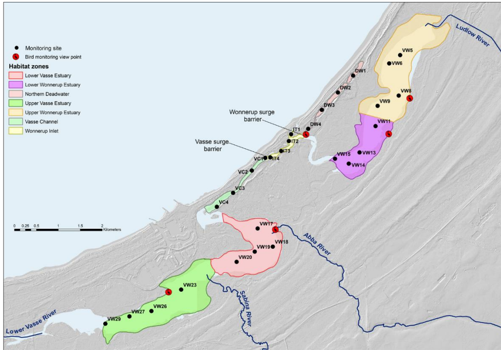
Figure 1. Map of the Vasse-Wonnerup showing the four sites sampled in each of the six regions in each season between March 2017 and March 2020. No sampling occurred in the Deadwater during the current study. Map supplied by the Department of Water and Environmental Regulation.
