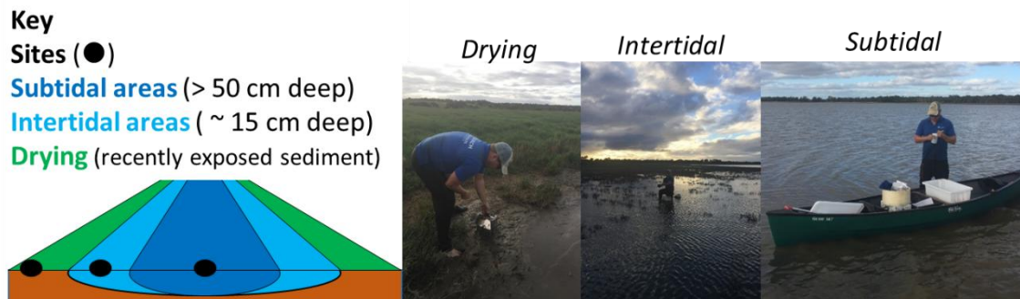
Figure 2. Conceptual diagram and photographs of the three water depths sampled at each site in the Upper Vasse Estuary and Upper Wonnerup Estuary regions during January and March of each year. Photos taken by Dr Linda Kalnejais.
